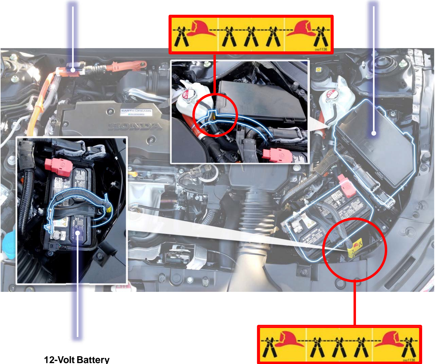
High-Voltage Cables
